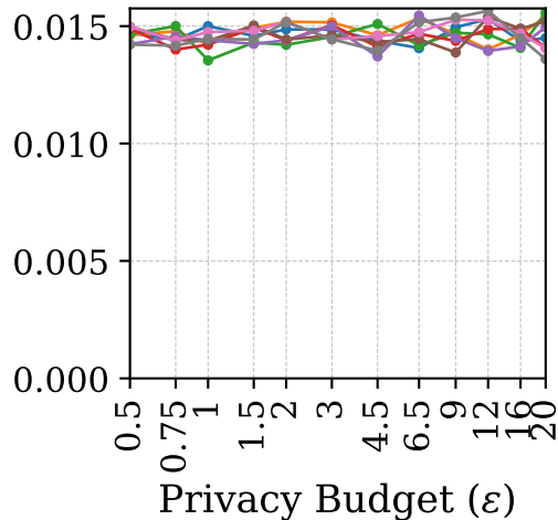
Link Prediction AUROC Error
