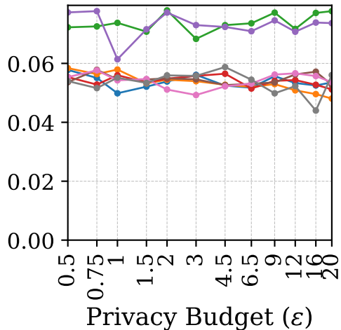
Link Prediction AUROC Error
